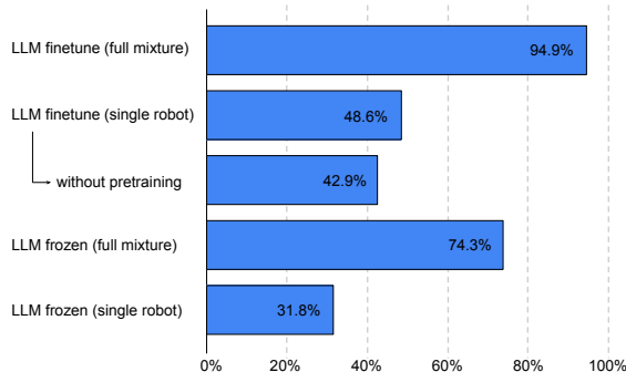
Figure 4: Planning success results in the TAMP environment (1% data) for PaLM-E-12B, comparing of the effects of PaLM-E models (i) using the full training mixture, (ii) pre-training (ViT and PaLM), and (iii) freezing or finetuning the language model. Transfer from full mixture is particularly effective. Note that full mixture contains only 1% of the training data (320 examples each) for the tasks evaluated here. Shown is the mean of tasks p_1 , p_2 .
